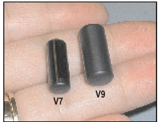
The V7-2L pinger has approximately half the volume and half the weight of the V9-6L pinger. The V7-2L weighs 0.75 grams in water and is 20 mm long.
